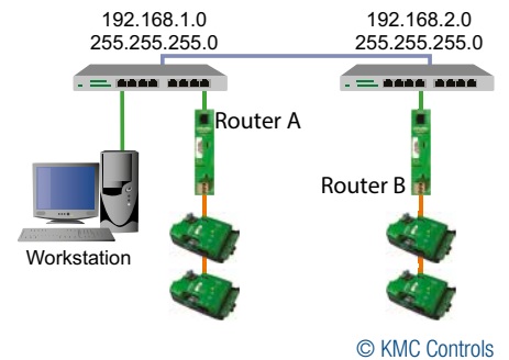
Figure 1: Internetwork with two subnetworks
